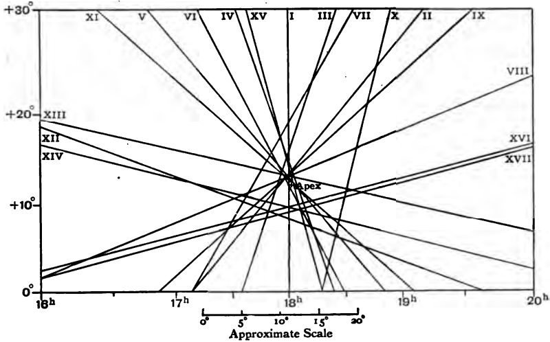
FIG. 10.—Convergence of the Directions of Drift I. from the 17 Regions.
